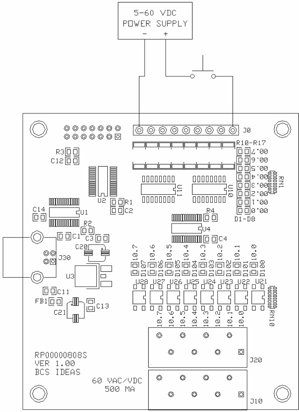
Push Button Input
